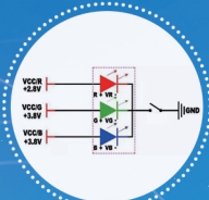
Common-Cathode
